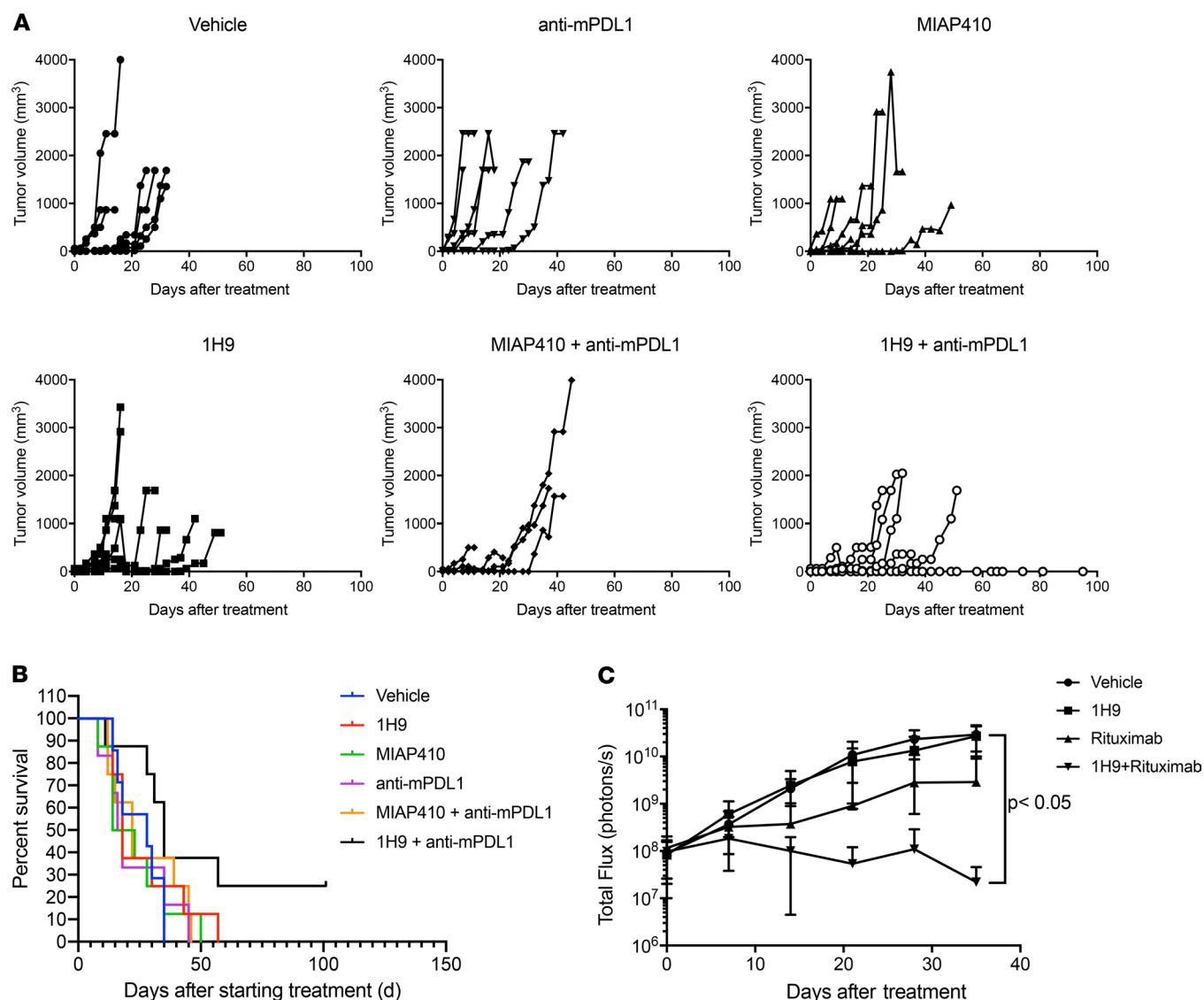
Figure 6. In vivo therapeutic activity of combination treatment with humanized 1H9. (A) B16F10 (2.5e5) cells were engrafted subcutaneously into CD47/SIRPα double-humanized mice ( n = 7 for PBS, 6 for anti-PD-L1, and 8 for the 1H9 and MIAP410 alone and in the combination groups). Twelve days after engraftment, treatment was initiated with PBS, 10 mg/kg of 1H9, anti-PD-L1 antibody, or MIAP410, or a combination of 1H9 and anti-PD-L1 antibody 3 times a week until the termination of the study. Caliper measurements were obtained 3 times per week during treatment and until the termination of the study to assess tumor burden and/or tumor recurrence. (B) Kaplan-Meier plot of overall survival of B16F10-engrafted cohorts. (C) Raji cells were engrafted subcutaneously into SIRPα-humanized immunodeficient mice ( n = 5 for each group). Ten days after engraftment, treatment was initiated with PBS, 10 mg/kg of 1H9, or rituximab, or a combination of 1H9 and rituximab 3 times a week until the termination of the study. Total flux measurements were obtained once per week during treatment and until the termination of the study to assess tumor burden and/or tumor recurrence. Statistics: repeated 1-way ANOVA with Holm-Šidák correction.
